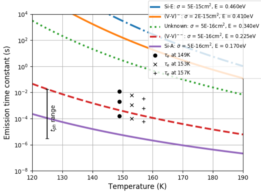
Figure 8. Emission time constants of different well-known defects as a function of temperature. The three peaks from the trap pumping data is shown as dots, x'es and plusses for 149 K, 153 K and 157 K, respectively. The vertical bar at 125 K shows the range of t_{ph} values used in these trap pumping tests.
