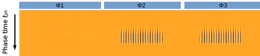
Figure 4. Dipole map of a three-phase device using the standard 1-2-3-1'-3-2-1 clocking scheme, showing that traps under phases 2 and 3 will pump in different directions, and that traps under phase 1 will not pump.
