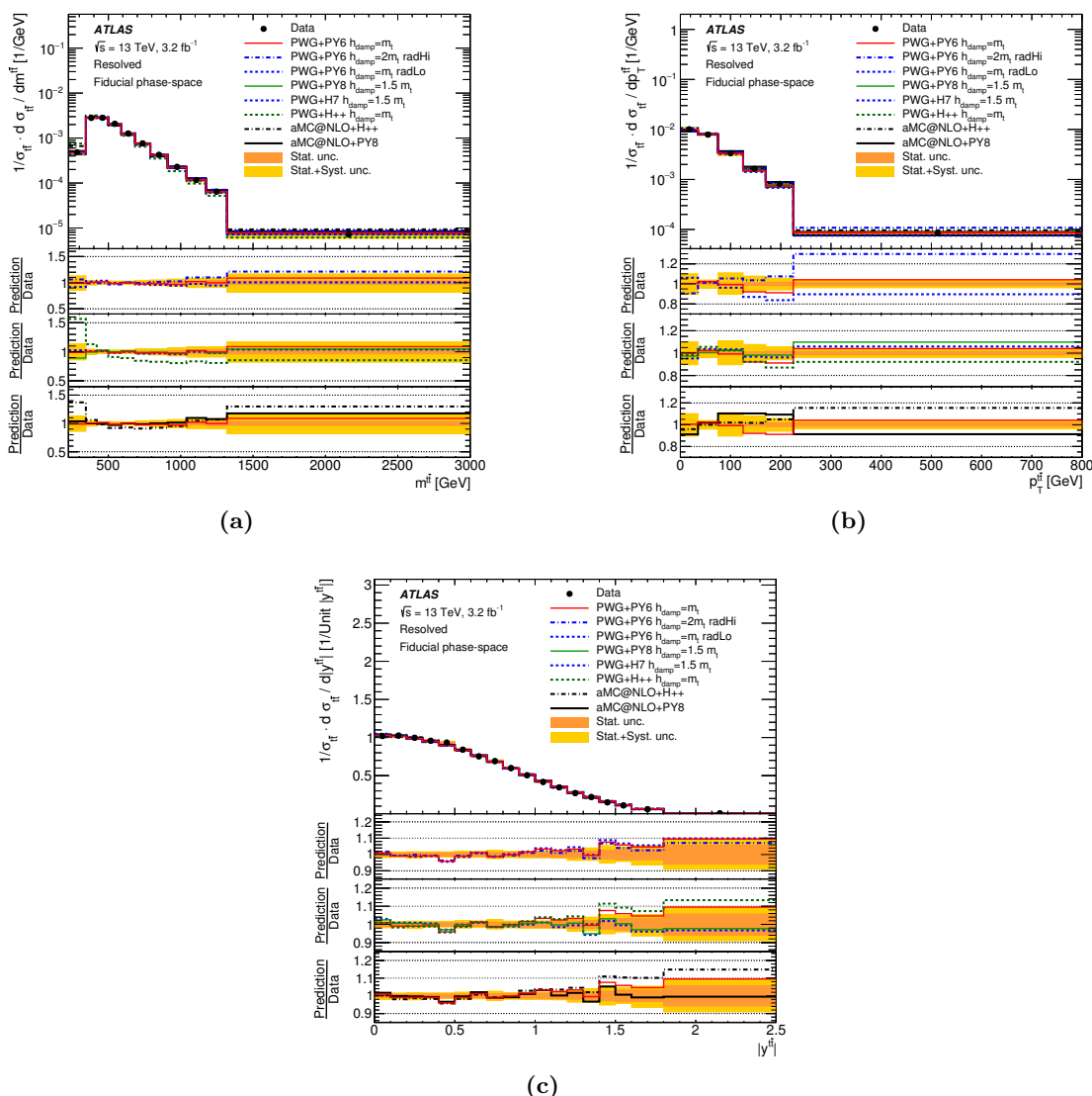
Figure 18. Fiducial phase-space relative differential cross-sections as a function of the (a) invariant mass ( m^{\text{tt}} ), (b) transverse momentum ( p_T^{\text{tt}} ) and (c) the absolute value of the rapidity ( |y^{\text{tt}}| ) of the t\bar{t} system in the resolved topology. The yellow bands indicate the total uncertainty of the data in each bin. The POWHEG+PYTHIA6 generator with h_{\text{damp}} = m_t and the CT10 PDF is used as the nominal prediction to correct for detector effects. The lower three panels show the ratio of the predictions to the data. The first panel compares the three POWHEG+PYTHIA6 samples with different settings for additional radiation, the second panel compares the nominal POWHEG+PYTHIA6 sample with the other POWHEG samples and the third panel compares the nominal POWHEG+PYTHIA6 sample with the MADGRAPH5_aMC@NLO samples.
