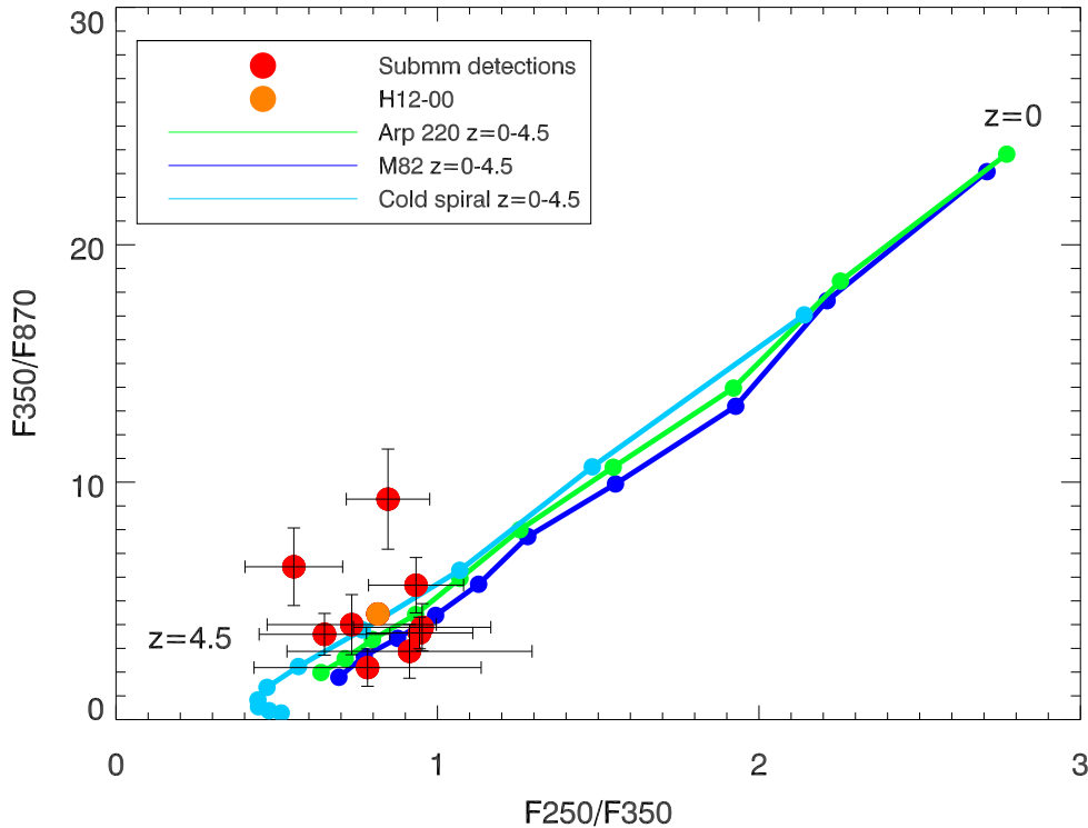
Figure 4. 250\ \mu\text{m}/350\ \mu\text{m} versus 350\ \mu\text{m}/870\ \mu\text{m} flux ratios of the sources detected in the submm classified as good, compared to colour tracks as a function of redshift for star forming galaxies. All these sources have colours similar to the lensed z = 3.26 source HATLAS12-00, which is the source in this figure with the smallest error bars, consistent with them all lying at a similar redshift. Template colour tracks are also shown, similar to those in Fig. 3.
