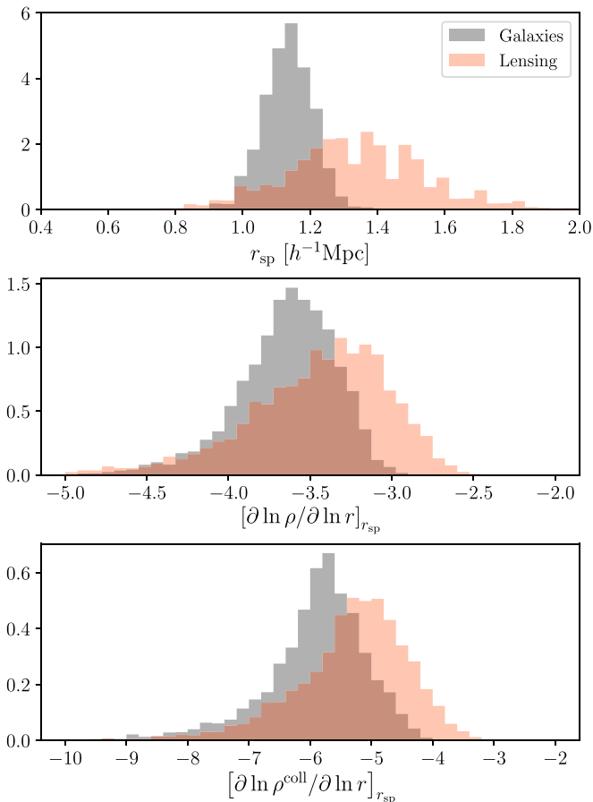
Figure 5. Top: posterior distributions of r_{sp} for galaxy density (gray) and lensing (red) data. Middle: posterior distribution of the slope of the total matter profile at r_{sp} . Bottom: posterior distribution of the slope of the collapsed matter at r_{sp} . All the distributions are marginalized over all nuisance parameters.
