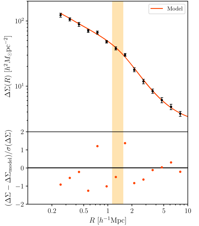
Figure 3. Top: lensing stacked excess surface mass density around DES REDMAPPER clusters with 0.2 < z < 0.55 and 20 < \lambda < 100 (black points with error bars). The red line shows the model fit to the measurements. The inferred 3D r_{\text{sp}} is shown as the vertical orange band, with the width of the band indicating the 1\sigma uncertainty. Bottom: difference in the model and the measurements divided by the uncertainty in the measurement.
