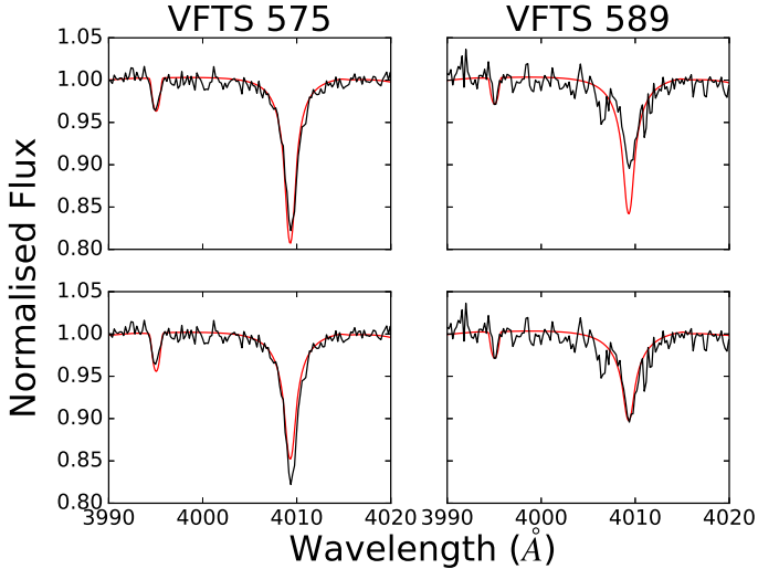
Fig. 2. Comparison of observed and theoretical spectra for the region near the N II line at 3995 Å. VFTS 575 and VFTS 589 are shown to the left and right respectively. The upper and lower panels have a 0% and 20% (with the theoretical spectra being scaled) contribution from the secondary,
