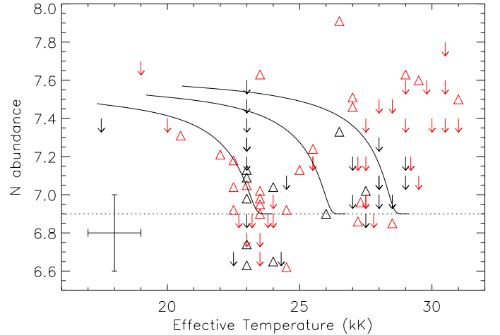
Fig. 5. Nitrogen abundance estimates (triangles) and upper limits (arrows) assuming no secondary flux contribution are plotted against effective-temperature estimates for our binary sample (black symbols). The representative error bars are for targets listed in Table 3, with those for targets from Table 4 being larger – see text for details. Also shown are the single-star sample discussed in Sect. 4.4.2 (red symbols – some targets have been moved slightly in effective temperature in order to improve clarity). The dotted line represents a baseline LMC abundance of 6.9 dex. The solid lines are evolutionary models from Brott et al. (2011a) with initial masses of 8, 10 and 12 M_{\odot} and an initial equatorial rotational velocity of approximately 230 \text{km s}^{-1} .
