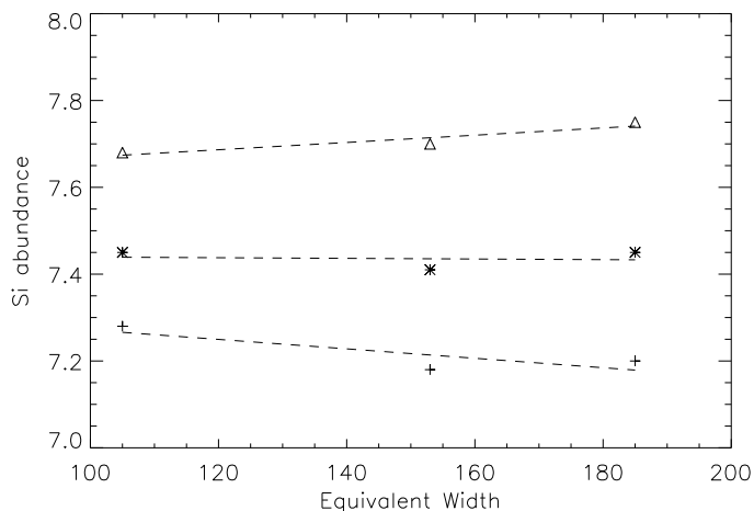
Fig. 1. An example of the estimation of the microturbulent velocity using the relative strengths of three Si III lines in VFTS 225. Abundances estimates are shown for v_t = 1 (triangles), 3 (stars) and 5 (crosses) \text{km s}^{-1} , together with linear least square fits.
