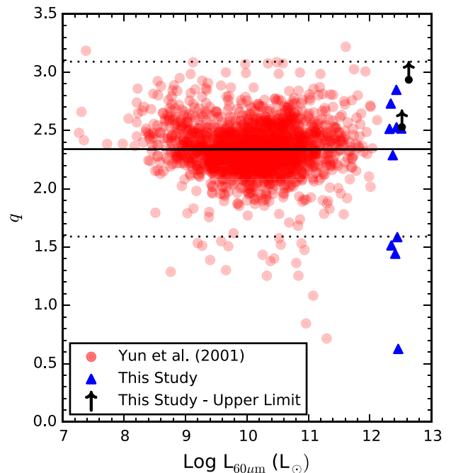
Figure 1. A comparison between the 60 μm luminosity and the derived q of sources from Yun et al. (2001) and this study. The solid horizontal line represents the mean q = 2.34 , as calculated by Yun et al. (2001). The dotted lines represent the radio-excess (below) and IR-excess (above) objects, defined as three times the standard deviation (SD) of q ( SD = 0.25 ) from the Yun et al. (2001) sample.
