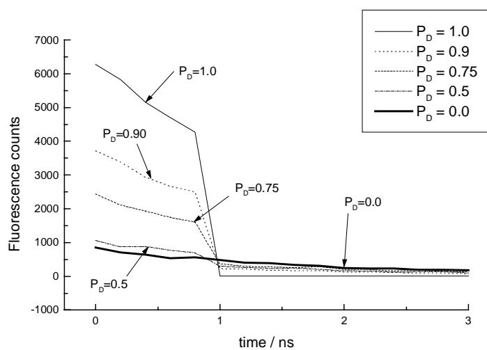
Figure 6: Simulated fluorescence photon distribution times for various DUMP probabilities compared with the UNDUMPED ( P_D=0 ) case. Molecular parameters in this case are: \tau_r = 2 ns, \tau_{ISC} = 1 μs, \tau_{TR} = 200 μs, PUMP-DUMP delay = 1ns. Significant enhancement is dependent on a high DUMP probability. Total enhancement I_D/I_U = 2.69, 1.80, 1.38, 0.75, 1.0 for P_D = 1.0, 0.9, 0.75, 0.5, 0.0 respectively.
