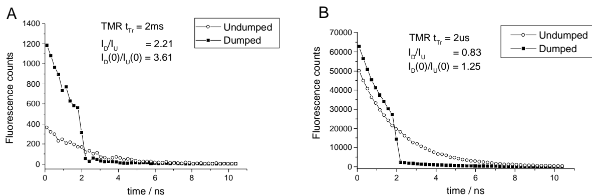
Figure 5: Plots of photon arrival times for DUMPED and UNDUMPED simulations of the fluorescence cycle for a single molecule with 2ms (A) and 2μs (B) triplet relaxation times. The enhancement of the total fluorescence yield I_D/I_U and the time zero intensities I_D(0)/I_U(0) are clearly greater for the longer triplet relaxation time.
