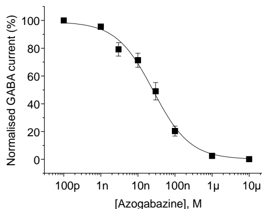
Figure 2. Concentration inhibition curve for azogabazine. Azogabazine was applied in combination with 10 \mu M GABA. pIC 50 : 7.646 \pm 0.141, n = 6 (IC 50 : 22.6 nM).
