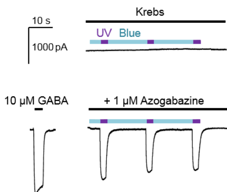
Figure 4. Whole-cell GABA currents recorded from \alpha 1\beta 2\gamma 2 GABA A receptors expressed in a HEK cell. Upper panel: cell exposed to Krebs and alternating periods of blue and UV light which do not induce current responses. Lower panel: The control 10 \mu M GABA current (left) is reduced in the presence of co-applied azobenzene, and GABA currents are only revealed by exposure to UV light (Right).
