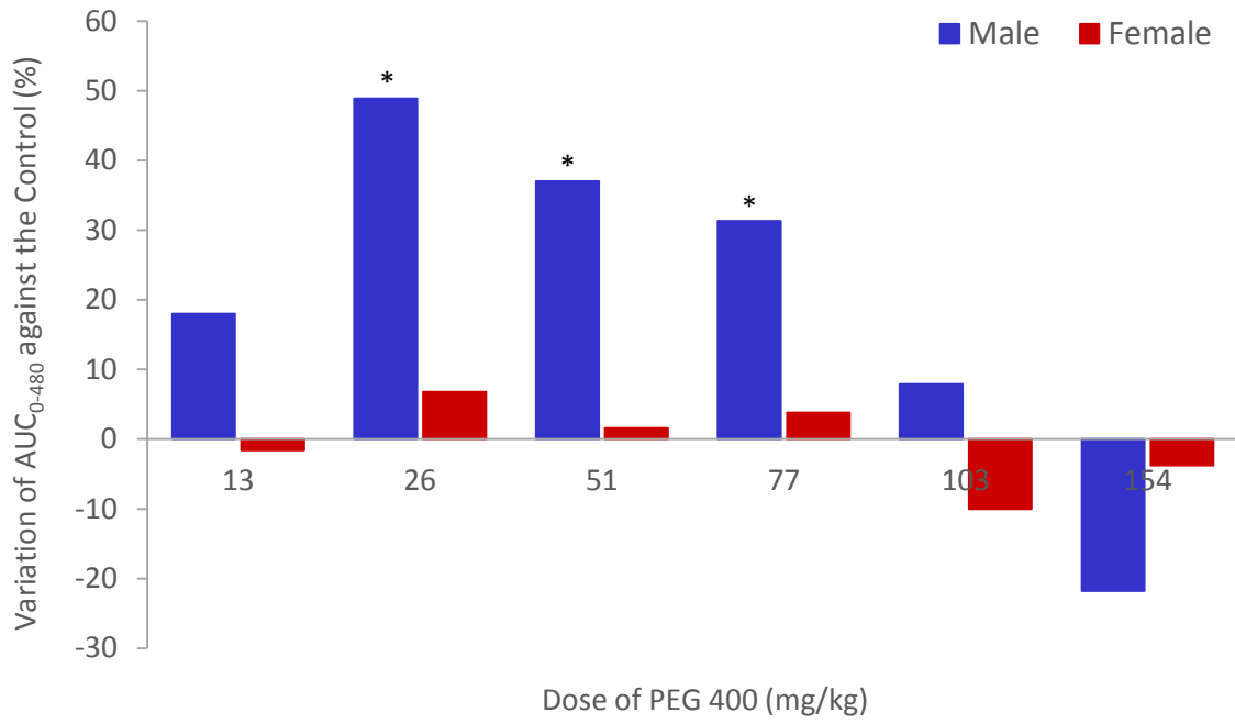
Figure 2 – Percentage difference in Ranitidine AUC 0-480 when compared to the control (0mg/kg PEG 400). * Denotes statistically significant difference compared to the control group (p<0.05).
