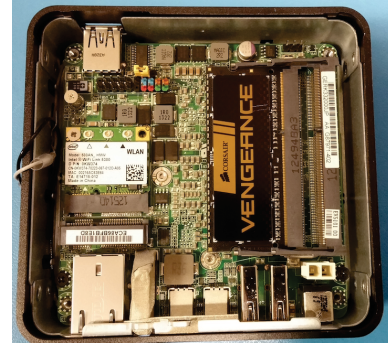
Figure 9: The inside of Phaser AP with one Intel 5300 card shown. Two NICs are employed to have a total of six available RF chains.
