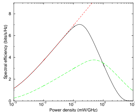
FIG. 5: Spectral Efficiency vs Input Power: Plots of i. Eq.(26)-solid black line; ii.Shannon formula, c = \log[1 + P/N] -short-dashed, red line; iii.Eq.(29)- long-dashed, green line.
