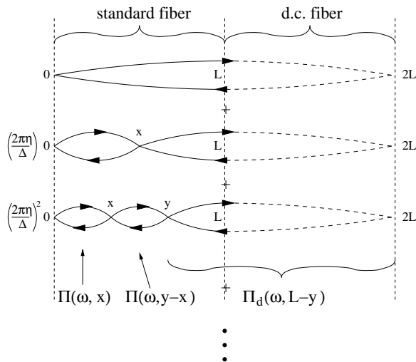
FIG. 4: Position-space diagrammatic series for \mathcal{G}_d^{II}(L, \omega) .
