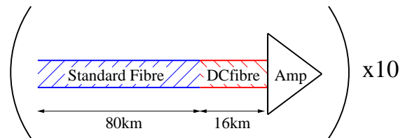
FIG. 1: Schematic Diagram of Optical Fiber System
