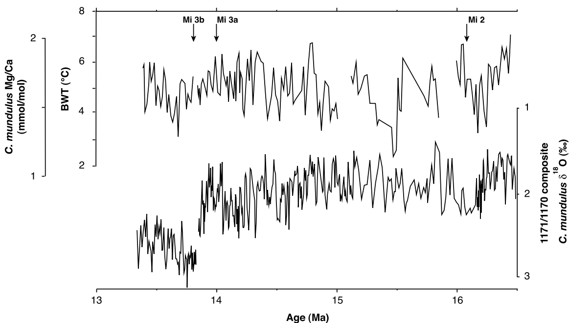
Figure 2. C. mundulus (top) Mg/Ca and (bottom) \delta^{18}\text{O} from ODP Hole 1171C ( 48^{\circ}30'\text{S} , 149^{\circ}06.69'\text{E} ; 2150 m) plotted versus age (a detailed discussion of the age model may be found in the text). Data were generated at 20 cm intervals (Mg/Ca) and at 10 cm intervals ( \delta^{18}\text{O} [Shevenell and Kennett, 2004]) from 150 to 205 meters below sea floor (mbsf). Each Mg/Ca data point represents an average of one to six analyses. Analytical reproducibility over the 18-month study, determined using consistency standards, is estimated at \pm 0.7\% ( 1\sigma ). Replicate analyses ( df = 65 ) were conducted on \sim 30\% of the samples. Precision of Mg/Ca data, estimated from the pooled standard deviation of the replicates, is \pm 9.8\% . Mi events of Miller et al. [1991b] are identified.
