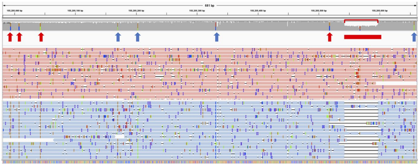
FIGURE 2 Detection and phasing of a 55-base pair exonic deletion in S5. The coverage track, with eight SNVs highlighted, and a selection of reads are shown, over exons 9 and 10 (chr1:155,204,981–155,205,661; NGMLR alignment). The deletion is clearly visible as a drop in coverage (red bracket). Reads are grouped and colored by haplotype for these variants, which are all on the blue-colored reads. The arrows point to the SNVs (red = coding, blue = noncoding) and the red box to the deletion. GenBank reference sequence NM_000157.3
