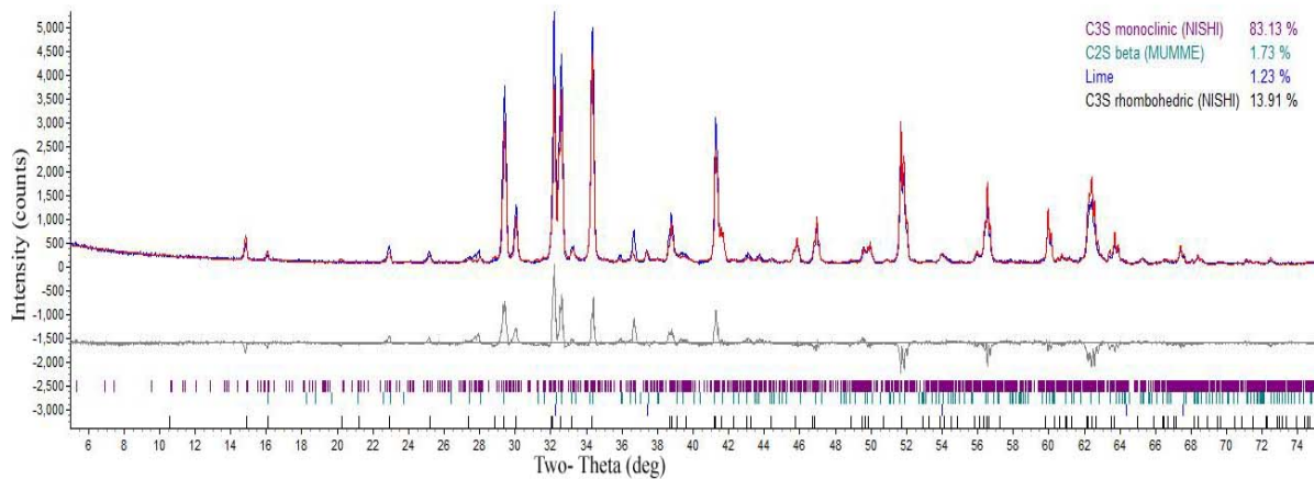
Figure 1. Rietveld plots for anhydrous C_3S sample with the observed (blue line), calculated (red line) and difference (bottom line) powder patterns.
