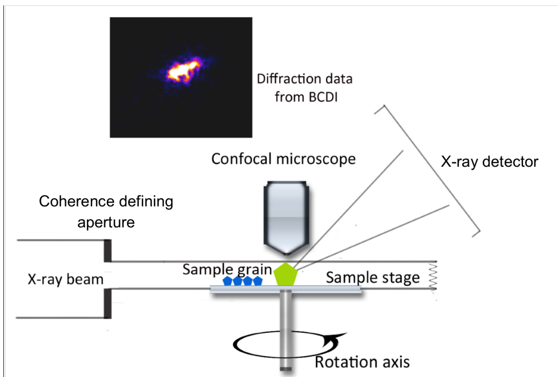
Figure 2. Schematic BCDI experiment setup at the beamline I-13 of the Diamond Light Source
