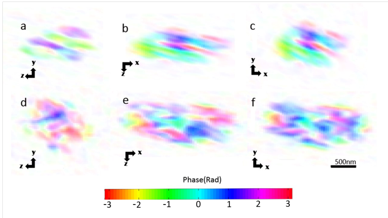
Figure 6. Cross sections of the grown calcite crystal after the hydrated C_3S sample was exposed to CO_2 for 8 hours (a, b, c) and 16 hours (d, e, f). The images were color-coded by the phase value using the HSV color scheme to illustrate the phase domains.
