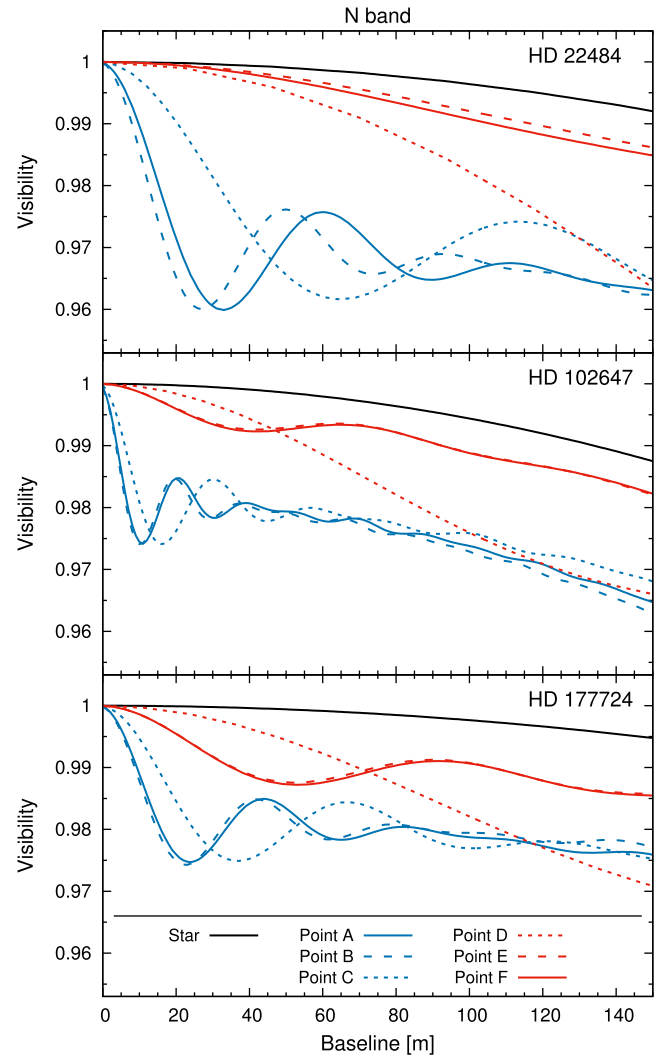
Figure 4. Same as Figs 2 and 3, but for the N band ( \lambda = 10 \mu\text{m} ).
